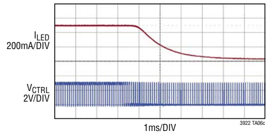
V CTRL Duty Cycle Stepped from 75% to 15%
