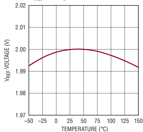
V REF Voltage
